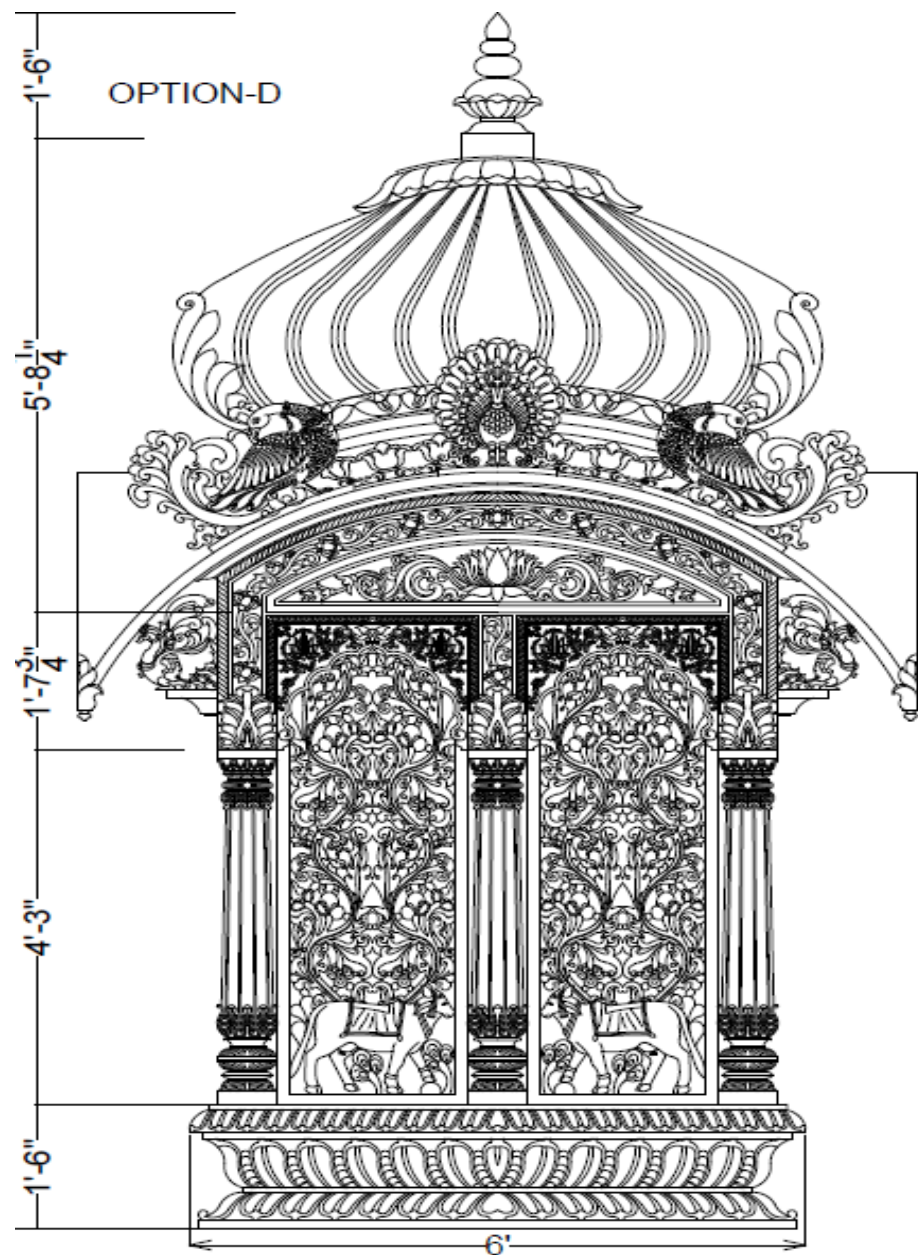
SIDE ELEVATION
